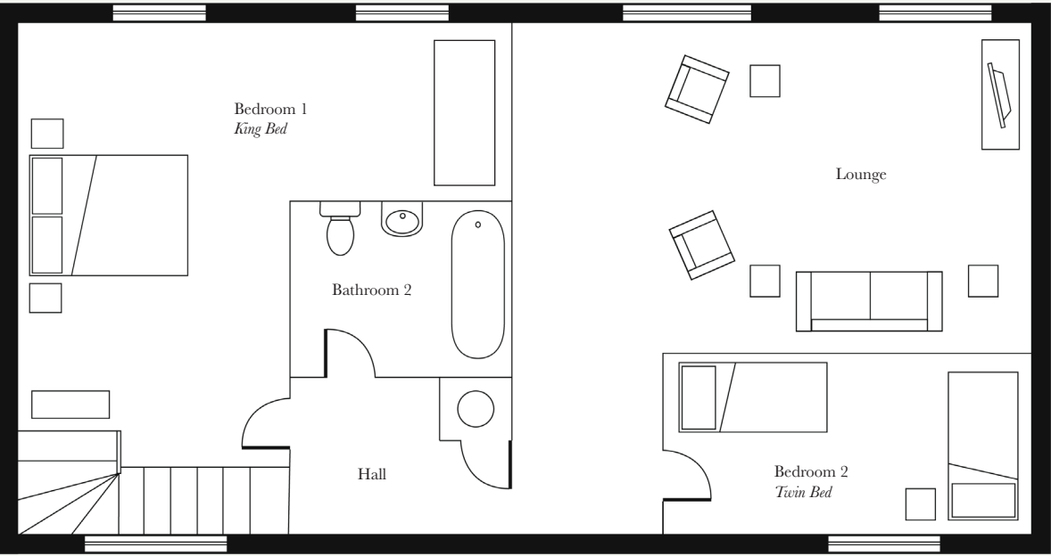
FIRST FLOOR
